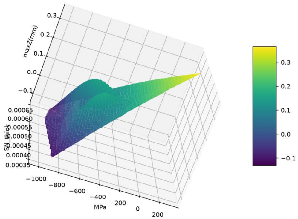
Surface Plot of maxZ vs MPa and SN_thick
